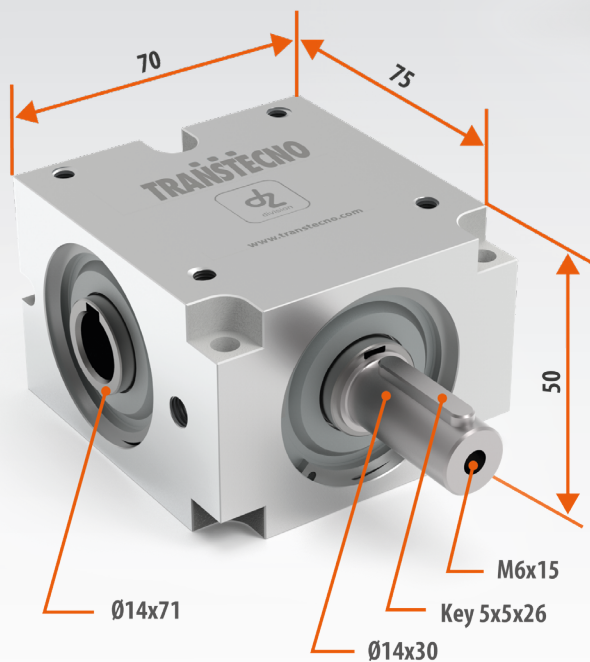
Input shaft + output shaft version BBIS503BC
