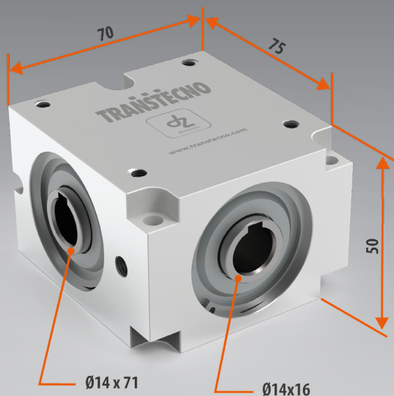
Input shaft + output shaft version BBIS503BC
