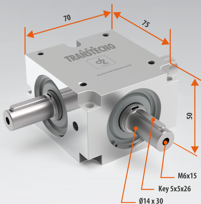
Input shaft + hollow output shaft version BBIS503U
